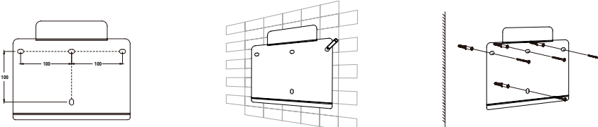
Figure 4 Dimensions of wall bracket
